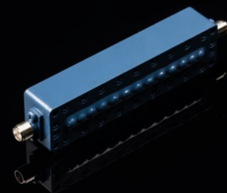
5.8 GHz Bandpass Filter Frequencies between 5150 MHz and 5850 MHz
