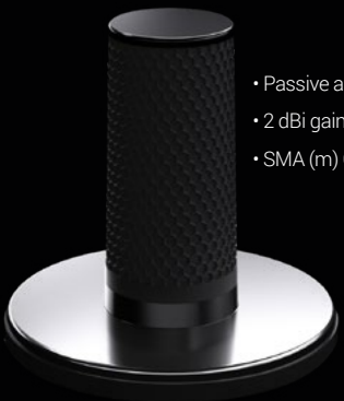
OmniLOG® PRO 1030H 100W Transmit/Receive Antenna - 700MHz - 3GHz
