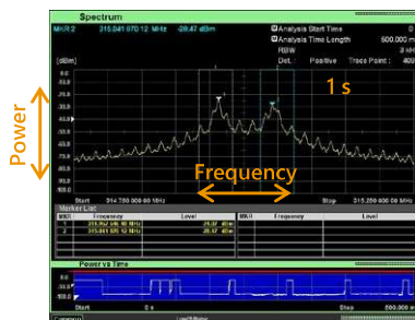
Trace display example (Frequency vs. Time)
