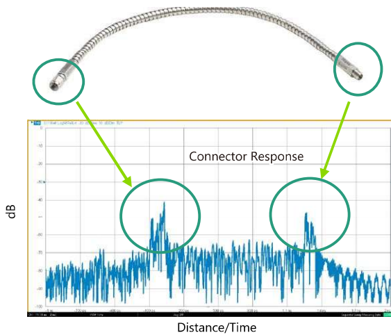
TDR data on a normal cable
