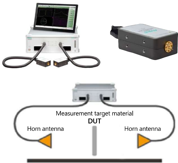
2-port Vector Network Analyzer (VNA) MS46522B-082 Frequency range: 55 GHz to 92 GHz
