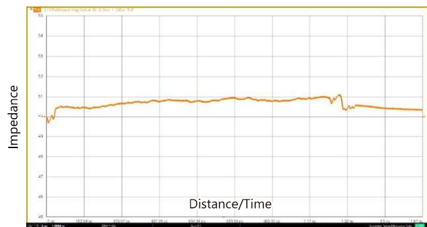
Measurement of input/output impedance and transmission loss, Characteristic impedance evaluation (TDR)
