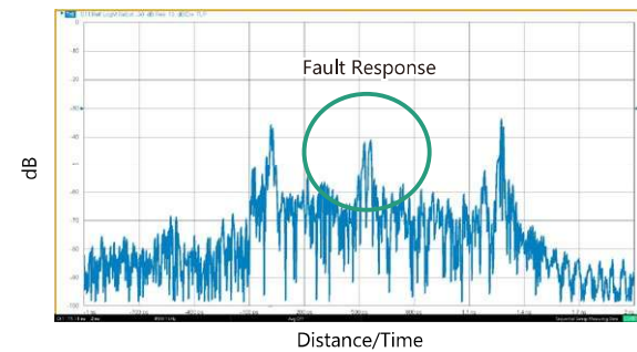
TDR data on faulty cable
