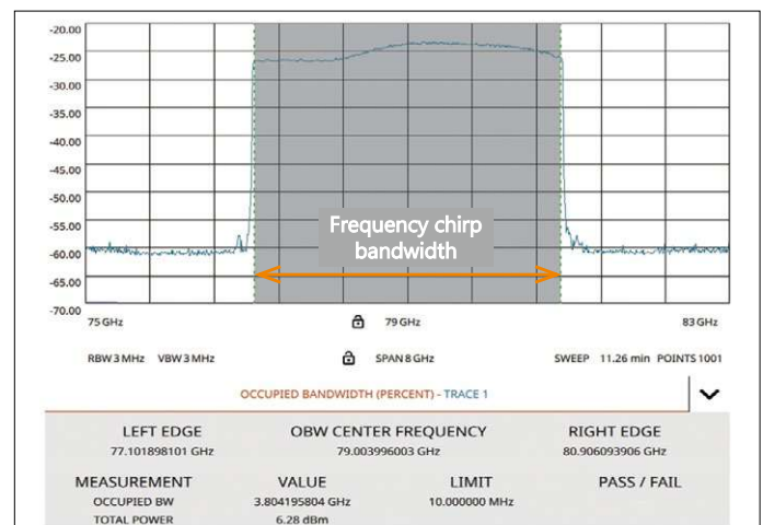
Radar chirp signal measurement example (signal level, frequency characteristics, bandwidth, upper and lower bandwidth frequencies, and center frequency)
