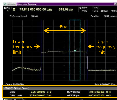
OBW Measurement Example
