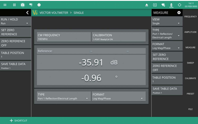
Log Mag and Phase
