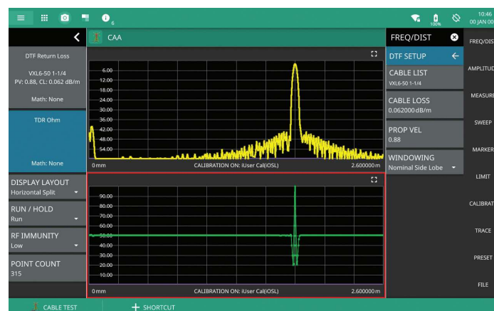
Split Screen Showing DTF and TDR Measurements
