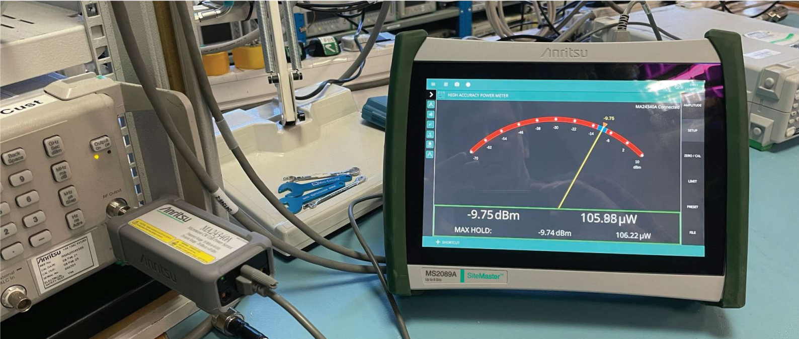
Site Master MS2085A/89A Supports Integration with USB Power Sensors for Maximum Measurement Accuracy
