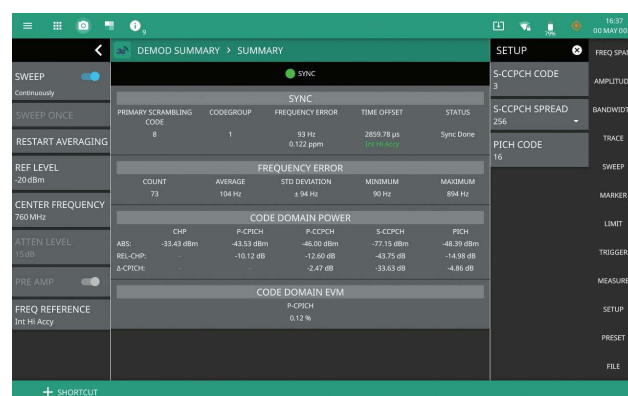
WCDMA Modulation Analysis Summary Screen
