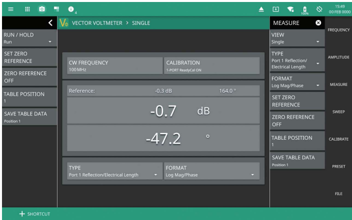
VVM Measurement of Phase Shift and Loss through DUT
