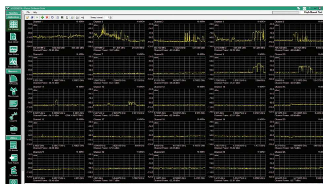
Use the High Speed Port Scanner Monitor Multiple RF Channels with a Single Site Master MS2089A on a Single PC Monitor
