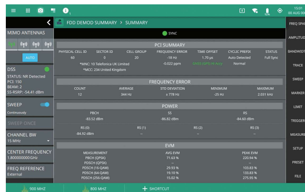
LTE Results Summary with DSS Detection Result Displayed in the Status Panel
