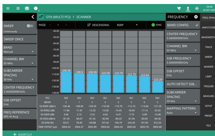
5G OTA Results
