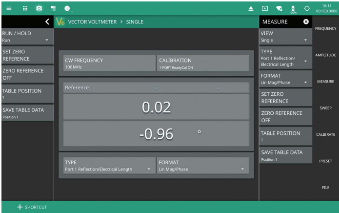
Linear Magnitude and Phase
