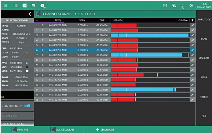
The Bar Chart Displays the Current Signal Level of Up to 20 Channels on a Single Screen
