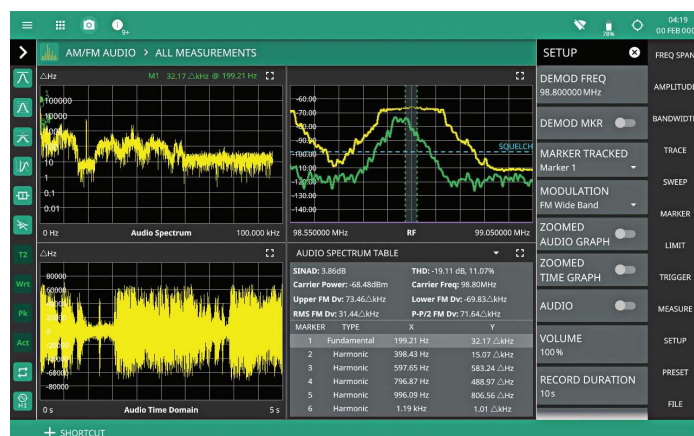
The AM/FM Modulation Measurements Screen Provides a Unique Simultaneous Display of Results and RF and Audio Spectrum
