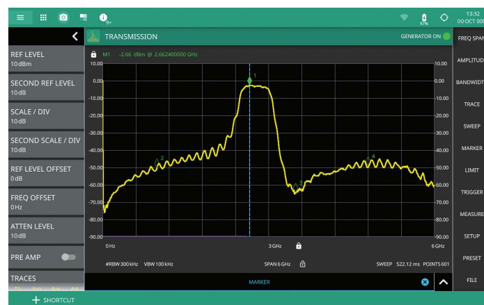
Bandpass Filter Measurement with Tracking Generator
