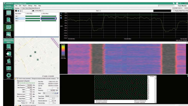
Vision Monitor Simultaneously Displays Current Spectrum, Spectrogram, and Pass/Fail History over an Extended Time Period on a Single Screen
