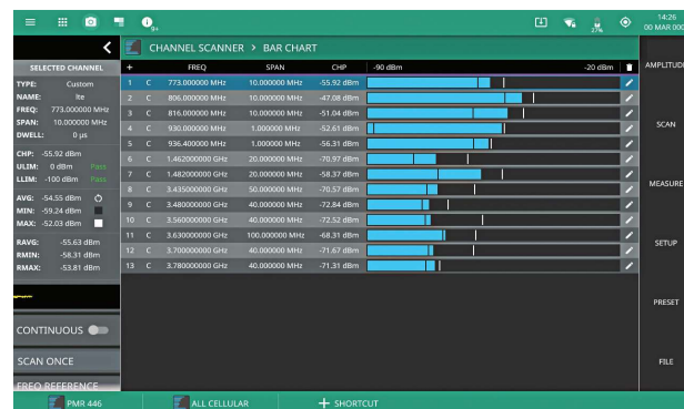
Bar Chart Display Monitoring GSM, LTE, and 5G Cellular Bands
