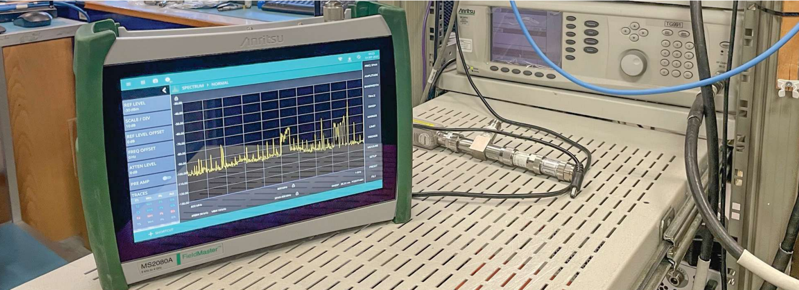
The RF Performance of the Field Master MS2080A Makes it Ideal for General Purpose Lab Applications
