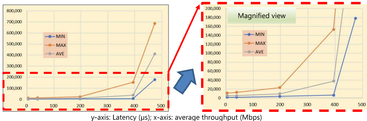
Figure 5. DL Latency Results Measured using MT1000A (UDP, 1482-byte packets)
