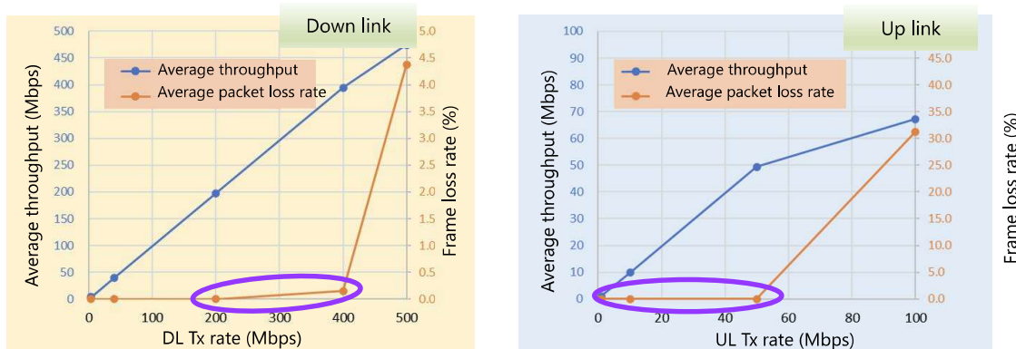
Figure 9. Traffic Load, Throughput and Packet Loss Rate (UDP, 1482-byte packets)
