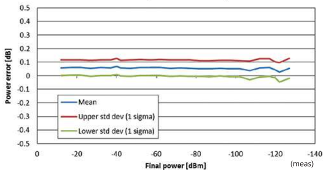
Linearity
