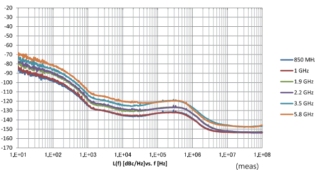
Single sideband phase noise
