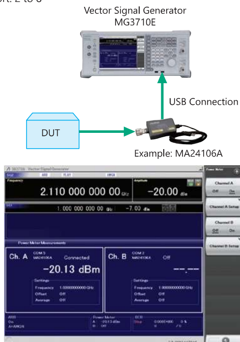
Power Meter Measurement Screen
