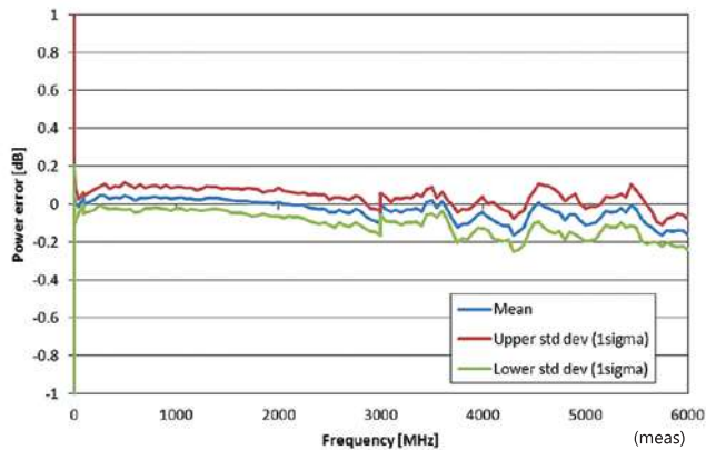
Frequency Characteristic
