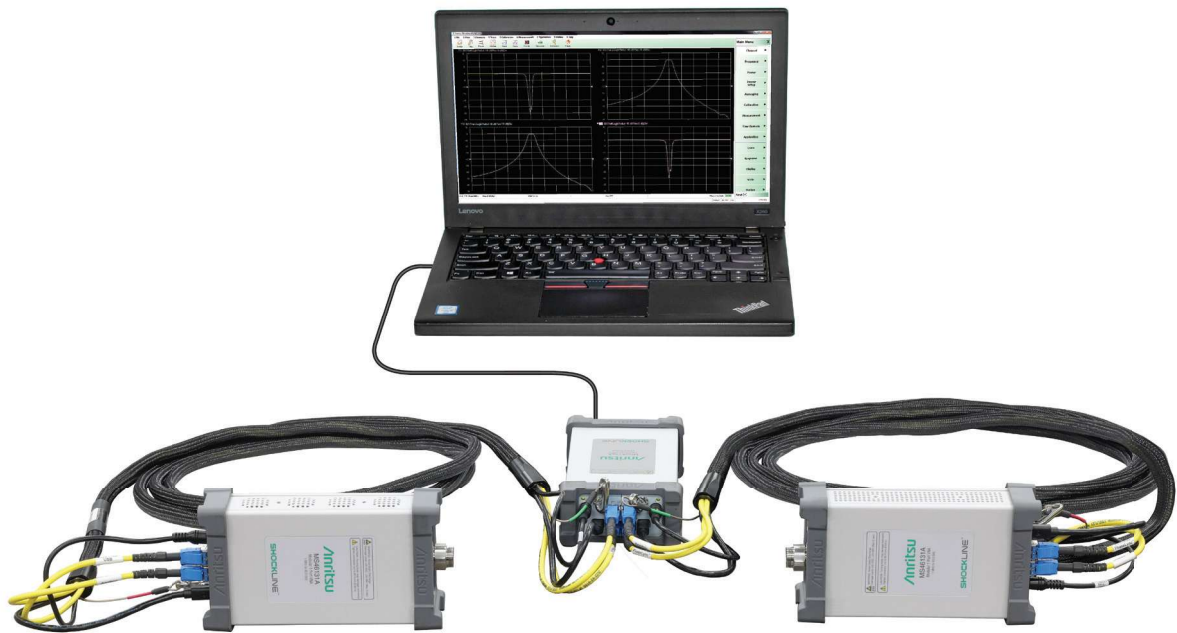
PhaseLync™ Enabled 2-port Distributed VNA ShockLine™ ME7869A
