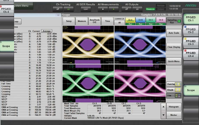
4ch NRZ Mask Margin Measurement
